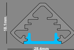
Perfil de Alumínio com Difusor e sem Barra Led Aluminium profile with Difusor, without Led
