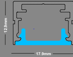
Perfil de Alumínio com Difusor e sem Barra Led Aluminium profile with Difusor, without Led
