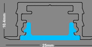
Perfil de Alumínio com Difusor e sem Barra Led Aluminium profile with Difusor, without Led
